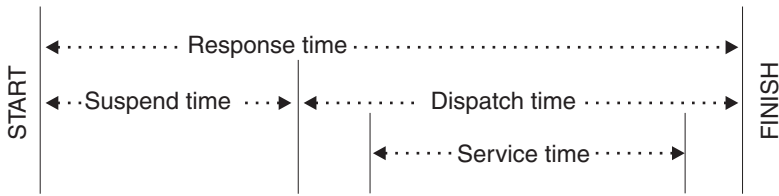
Figure 6. CICS internal response-time elements
